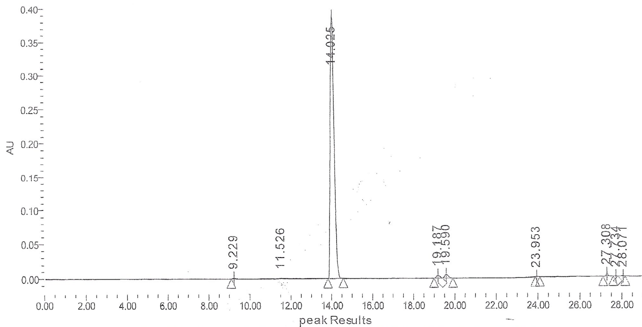
Auto-Scaled Chromatogram
